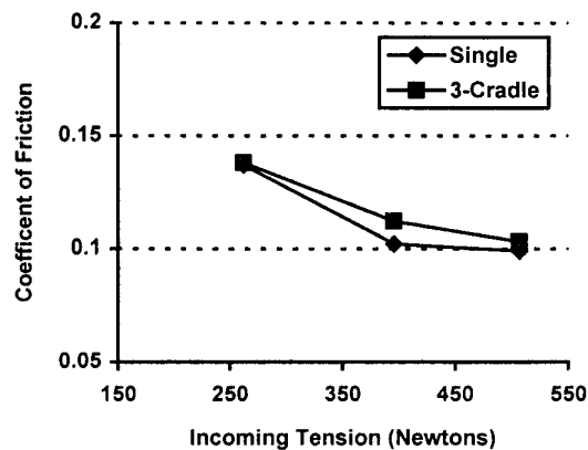
Fig 3. 2/0 Cable; Lubricated
