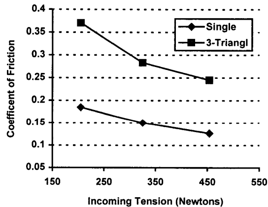
Figure 4. 400 MCM; Lubricated
