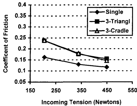
Figure 5. 350 MCM - Lubricated
