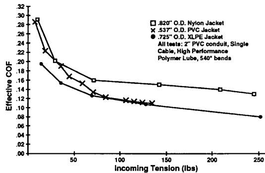
Figure 4. Three different types of cable (jacket) pulled through same conduit
