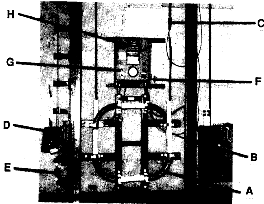
Figure 1. Multi-bend pulling device
